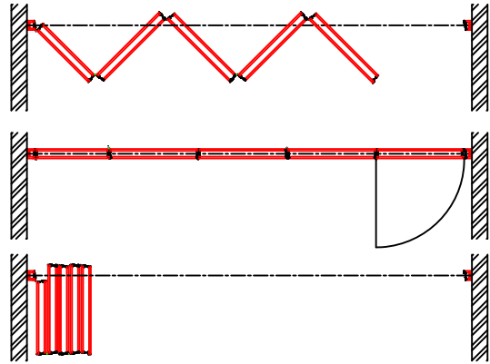
End Folding - Single Wing
